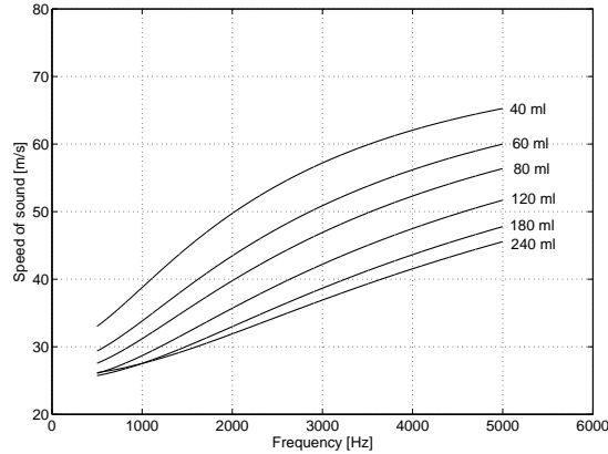
FIGURE 6. Speed of sound for varying porosity corresponding to the measurements in [5]. The fitted parameter values \sigma^{\text{static}} = 5.25 \cdot 10^6 \text{ kg/m}^3 \text{ s} , \alpha_\infty = 26.5 , \Lambda = 4.02 \cdot 10^{-4} \text{ m} are used.
