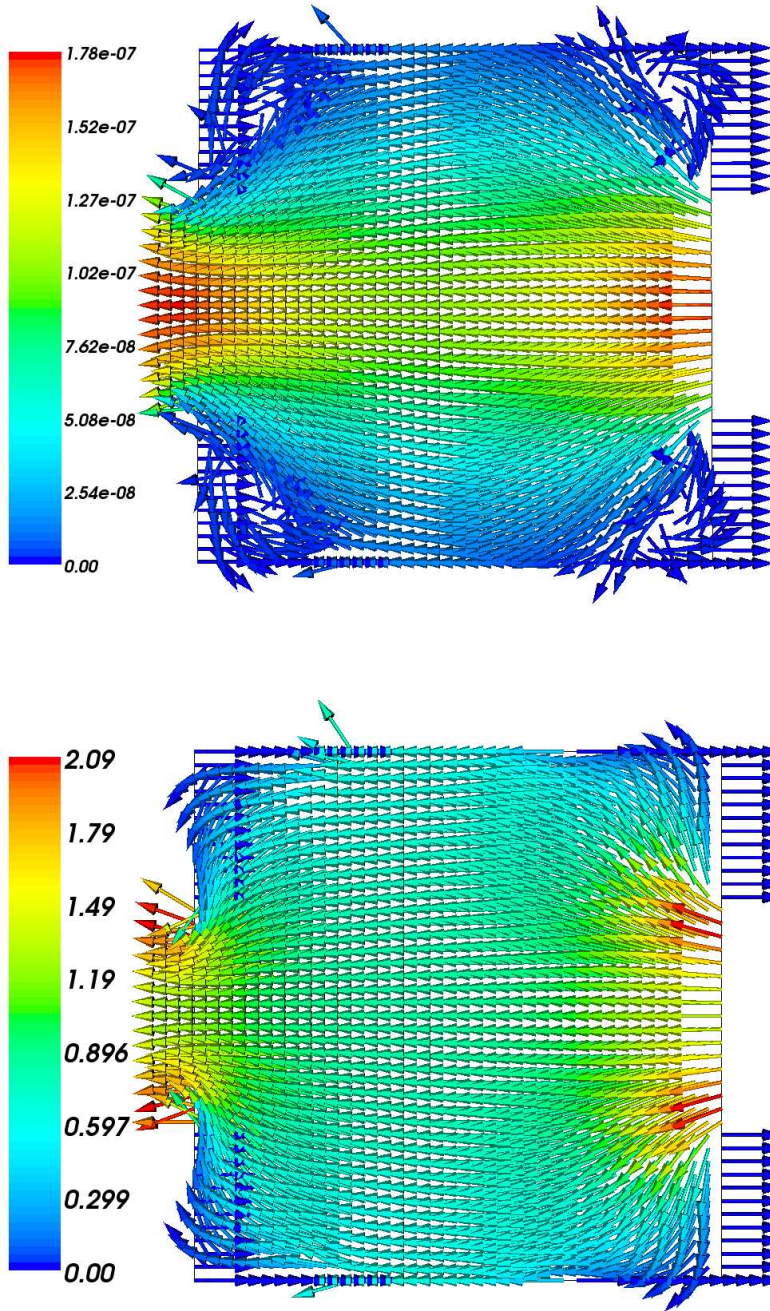
FIGURE 2. Above, the real part of \hat{w} is plotted for \omega = 10\text{s}^{-1} (top) and \omega = 10^6\text{s}^{-1} (bottom). This quantity corresponds to the instantaneous displacement field at t = 0 . In both cases, a = 0.2 . The above plots were obtained on a 40 \times 40 triangular mesh (a finer 128 \times 128 triangular mesh was used when computing \bar{Y}(\omega) ). The rightward pointing arrows along parts of the cell boundary is due to that the plot program plots an arrow directed along the positive \hat{y}_1 axis for zero-valued points.
