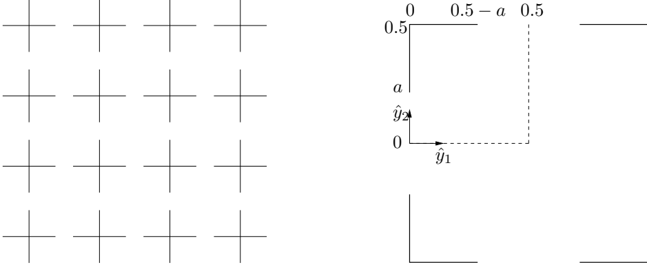
FIGURE 1. Left; A 2D idealized micro-scale geometry. Each micro-scale cell is quadratic. The cells are separated by infinitely thin wall, and connected by an opening in the middle of each of the walls. Right; The geometry of a single cell. The sides of the quadratic cell are of unit length in the (\hat{y}_1, \hat{y}_2) -coordinate system. Centered around the middle of each wall is an opening of width 2a . The dashed lines indicate lines of symmetry.
