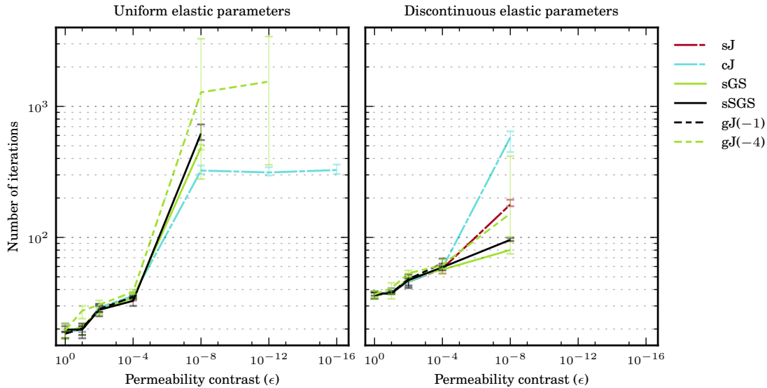
(b) The preconditioning methods that fail to converge for small values of \epsilon (large jumps in permeability)
