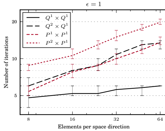
Figure 2: Iteration count for the homogeneous-domain problem. The sJ preconditioner was used. Q denotes quadrilaterals and P denotes simplices of a given polynomial order.
