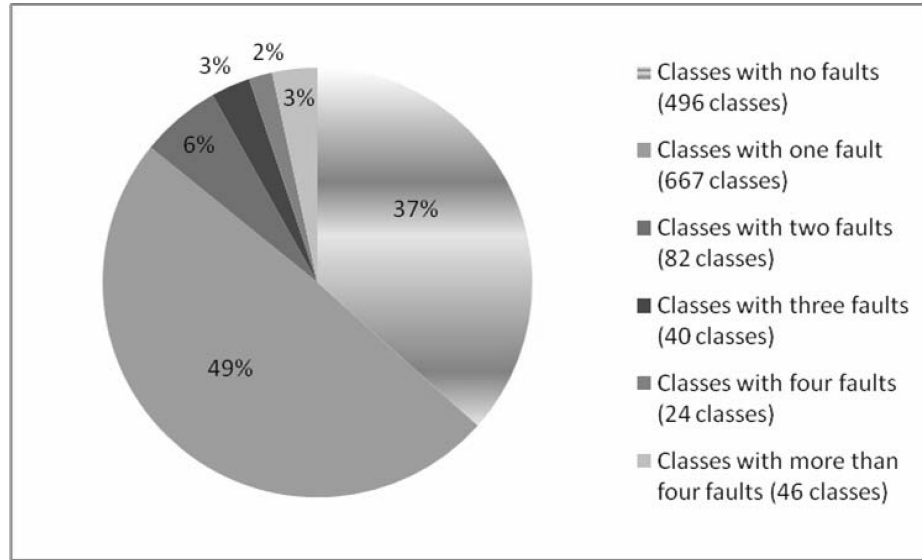
Fig. 4. The distribution of the number of faults detected in classes.
