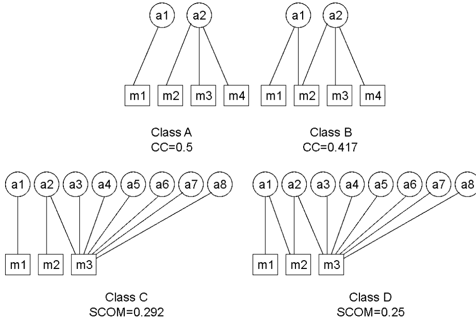
Fig. 2. Classes with different method-method connectivity patterns.
