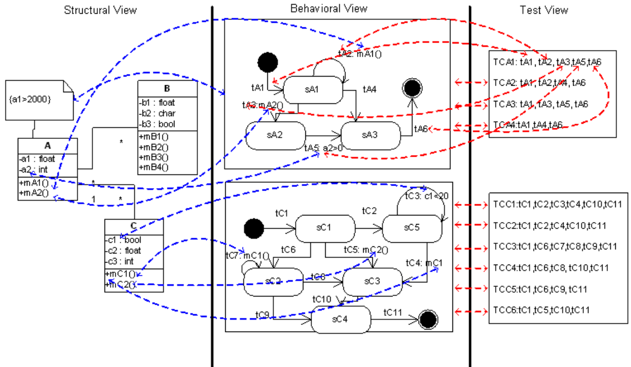
Figure 1. Relations between structural, behavioural and test view
