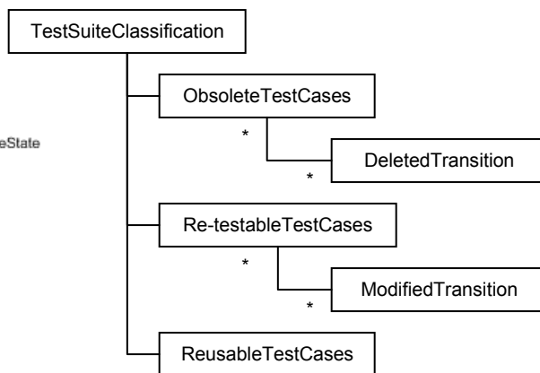
Figure 4. State-based Test Suite Classification
