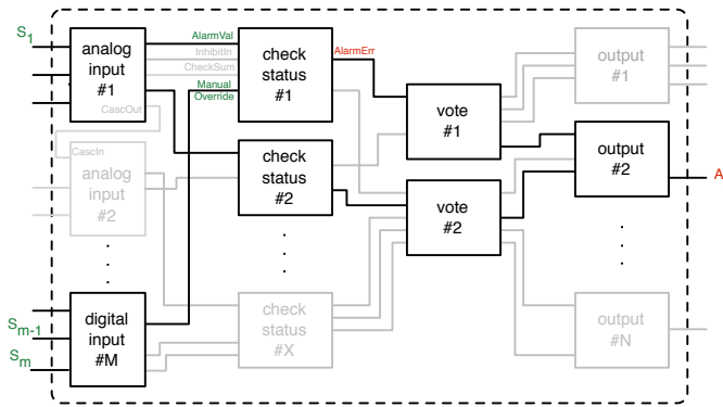
Fig. 4. System Information Flow highlighted for A_j in example system.
