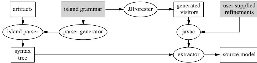
Figure 5. MANGROVE instantiation that allows processing in JAVA.
