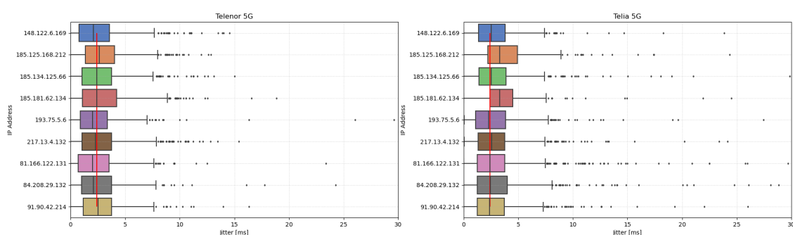
Figur 6.8: Jitter per server.
